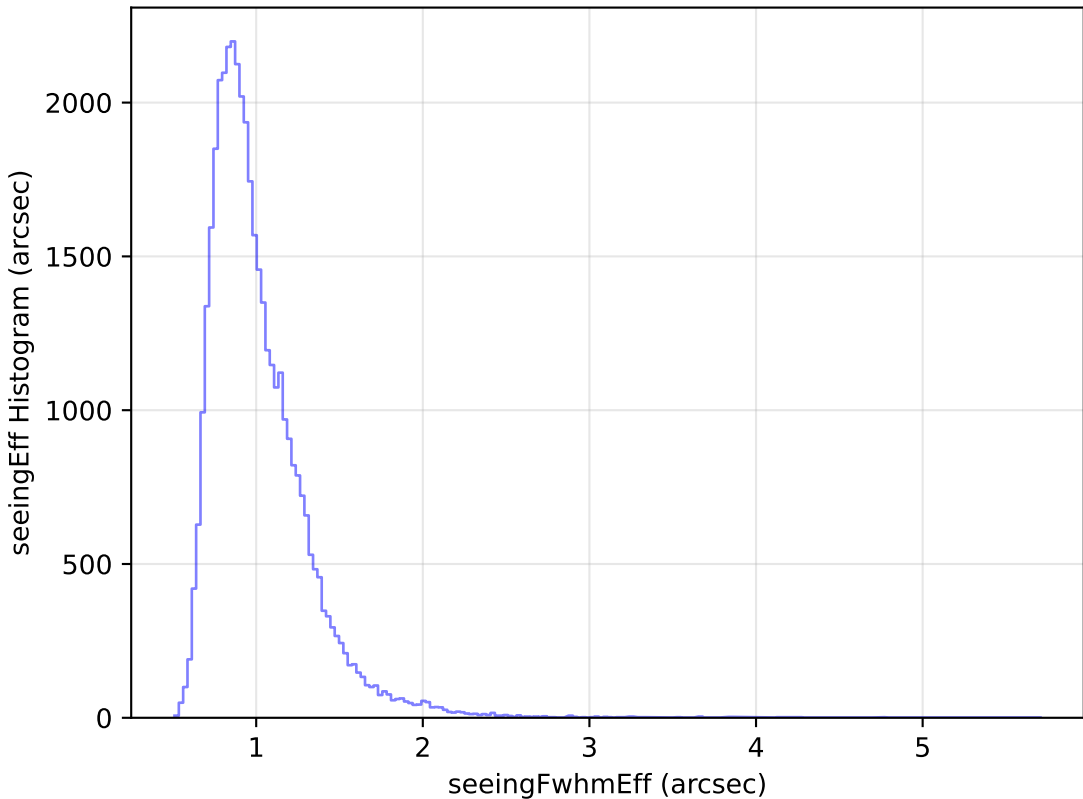
internal_u_expt60_nscale1.5v3.4_10yrs Yr 1 z band: seeingEff Histogram
