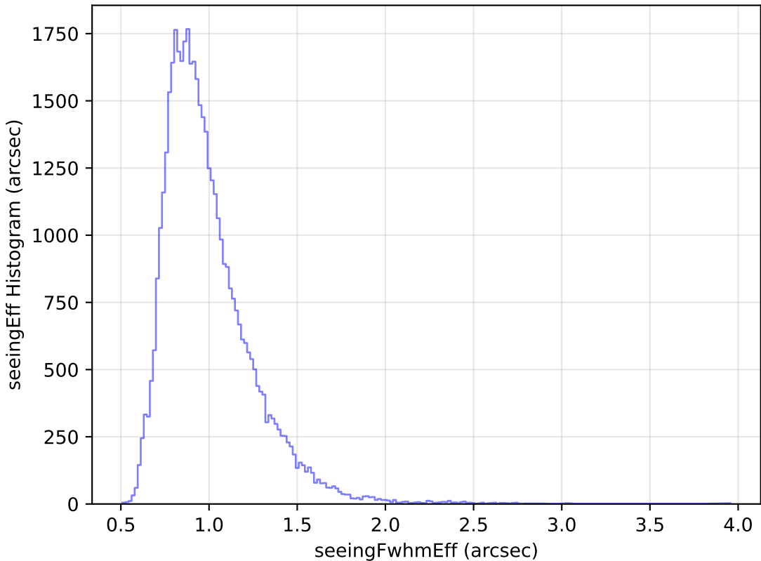
internal_u_expt60_nscale1.5v3.4_10yrs Yr 1 y band: seeingEff Histogram
