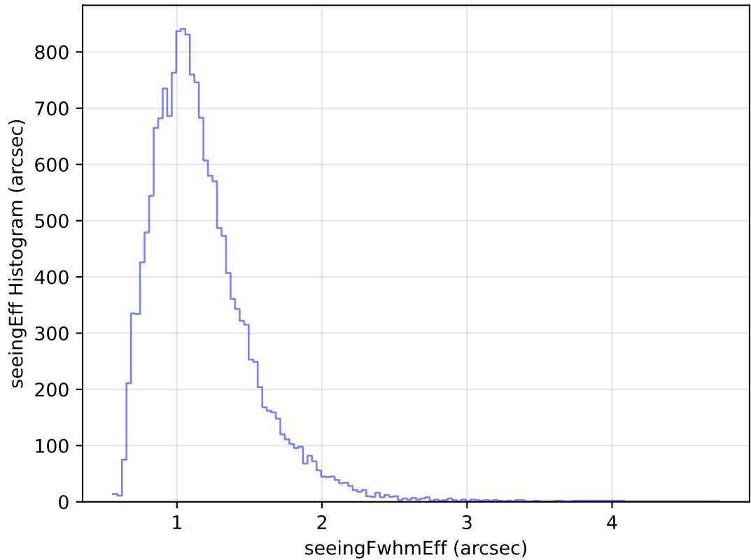
internal_u_expt60_nscale1.5v3.4_10yrs Yr 1 u band: seeingEff Histogram
