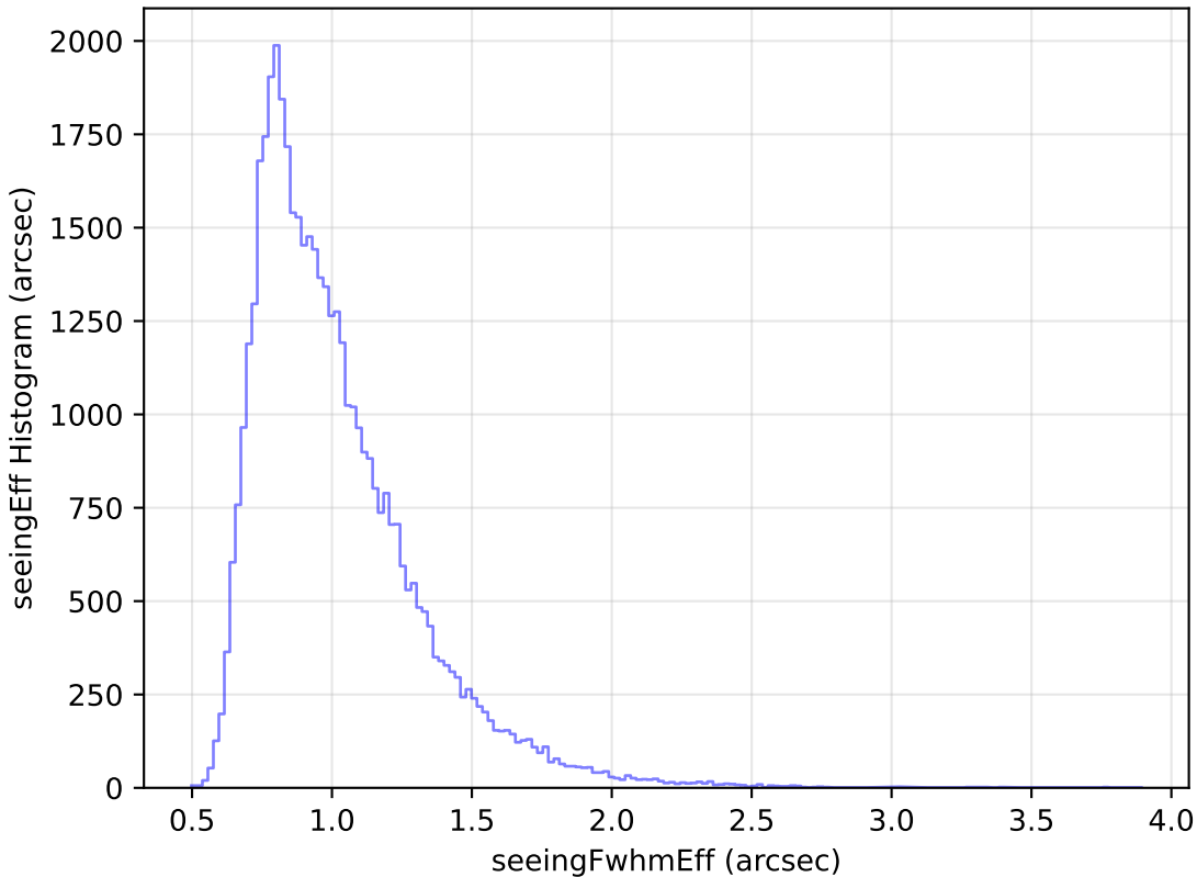
internal_u_expt60_nscale1.5v3.4_10yrs Yr 1 r band: seeingEff Histogram
