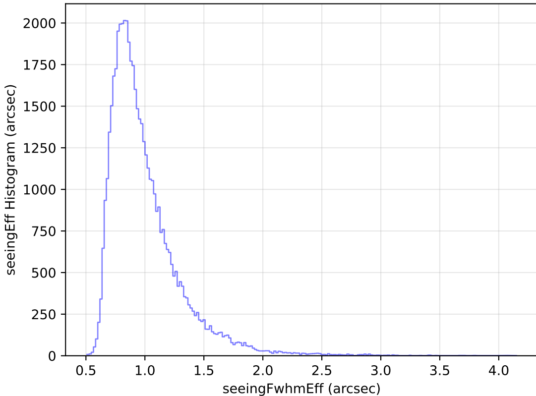
internal_u_expt60_nscale1.5v3.4_10yrs Yr 1 i band: seeingEff Histogram
