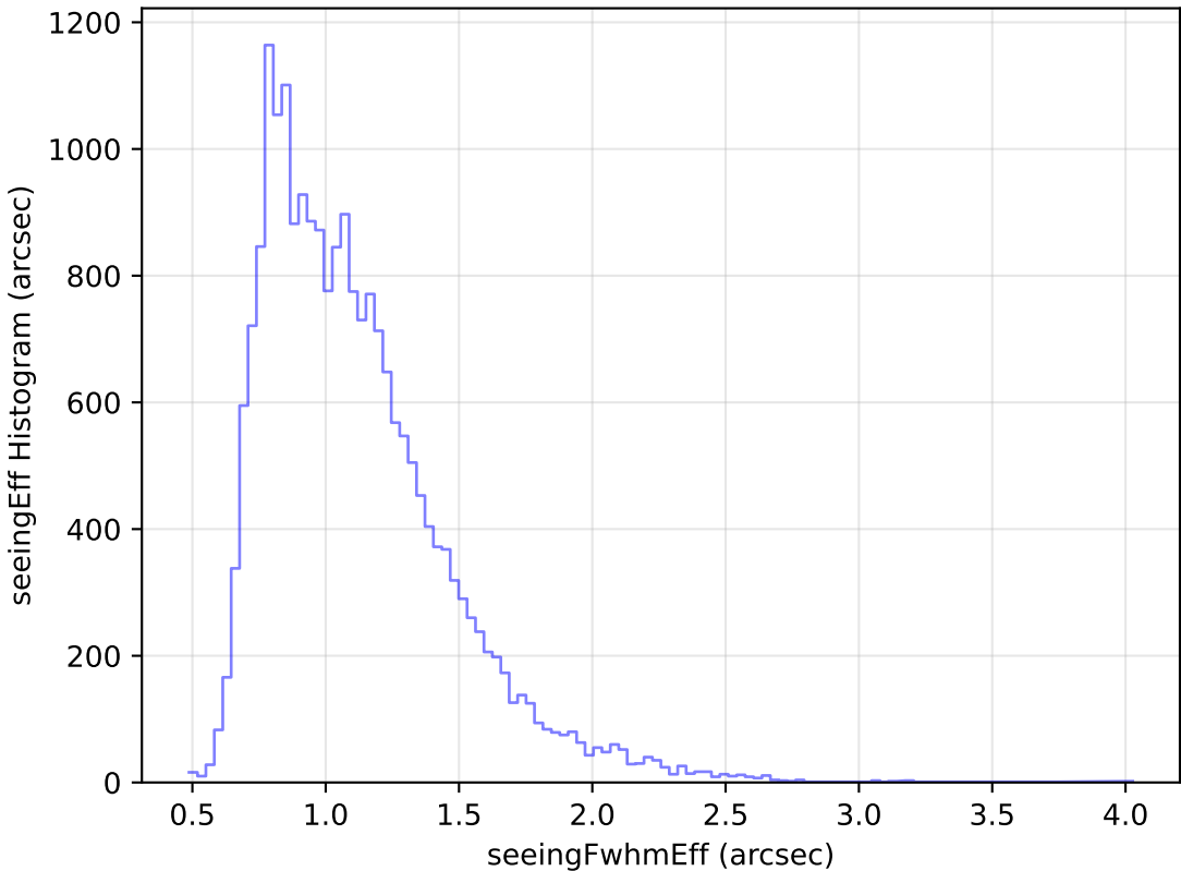
internal_u_expt60_nscale1.5v3.4_10yrs Yr 1 g band: seeingEff Histogram
