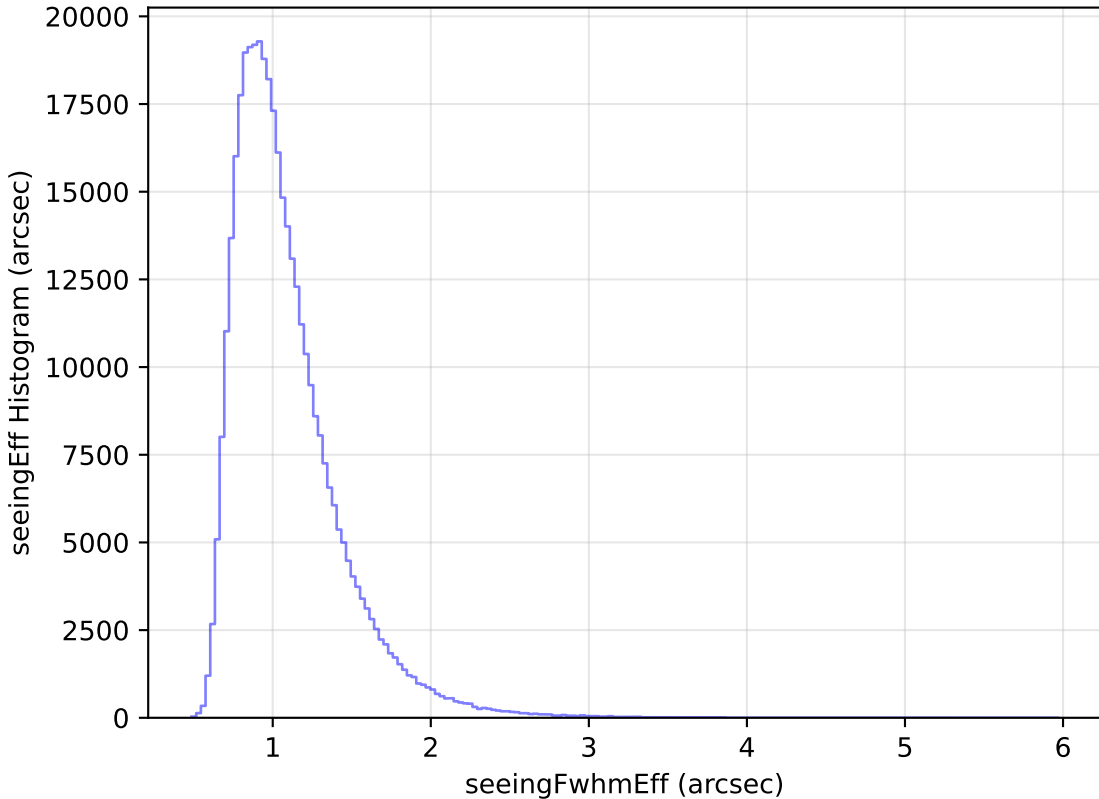
internal_u_expt60_nscale1.5v3.4_10yrs WFD z band: seeingEff Histogram
