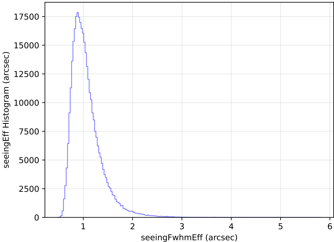
internal_u_expt60_nscale1.5v3.4_10yrs WFD y band: seeingEff Histogram
