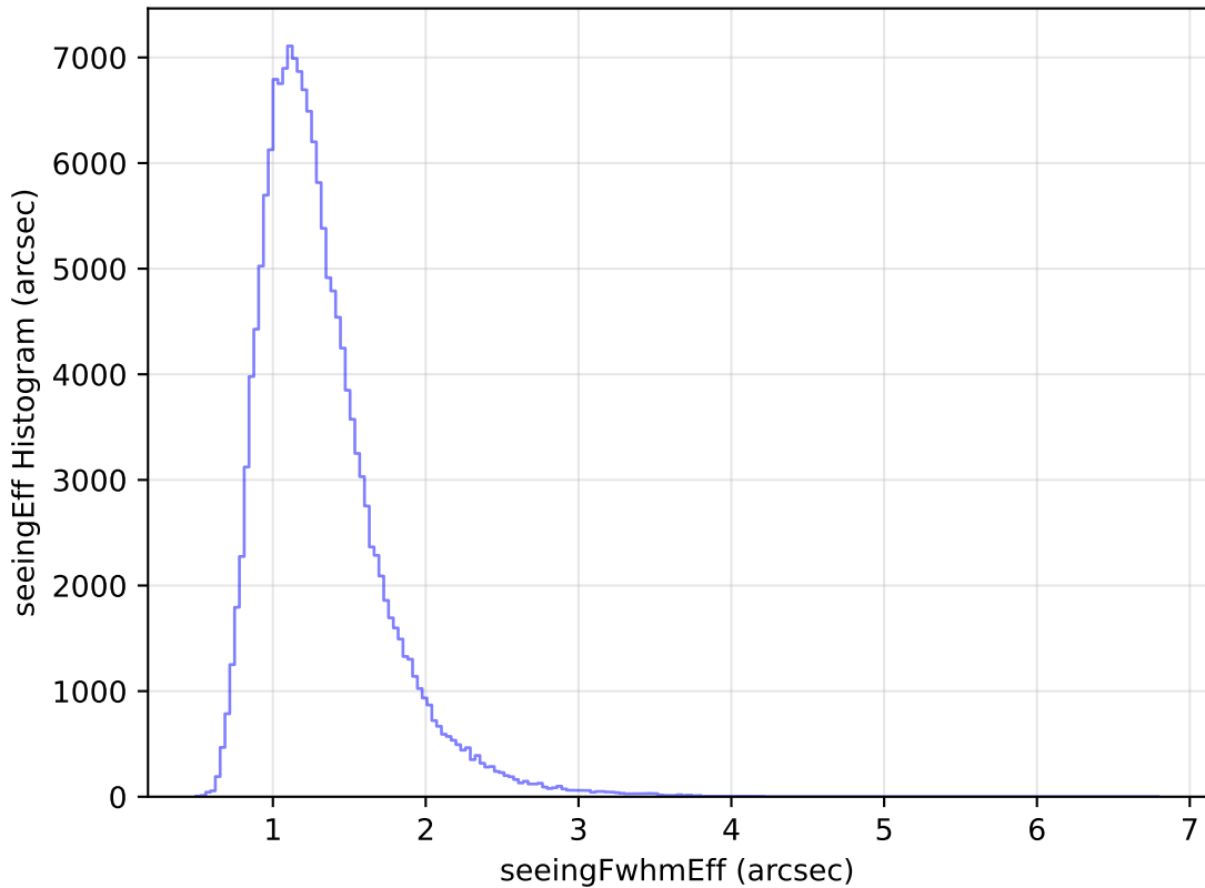
internal_u_expt60_nscale1.5v3.4_10yrs WFD u band: seeingEff Histogram
