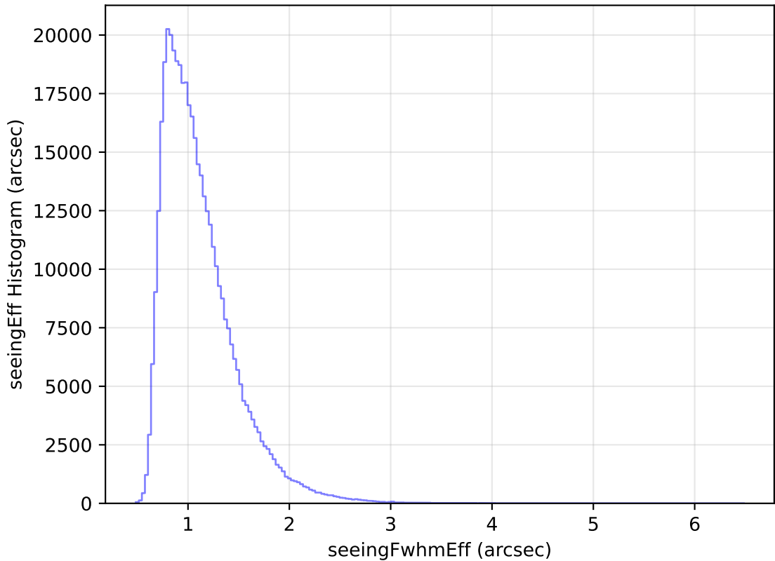
internal_u_expt60_nscale1.5v3.4_10yrs WFD r band: seeingEff Histogram
