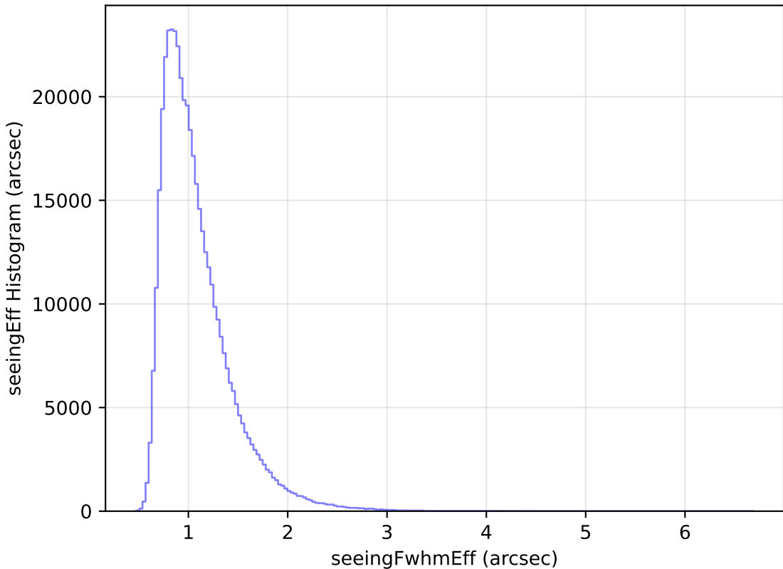
internal_u_expt60_nscale1.5v3.4_10yrs WFD i band: seeingEff Histogram
