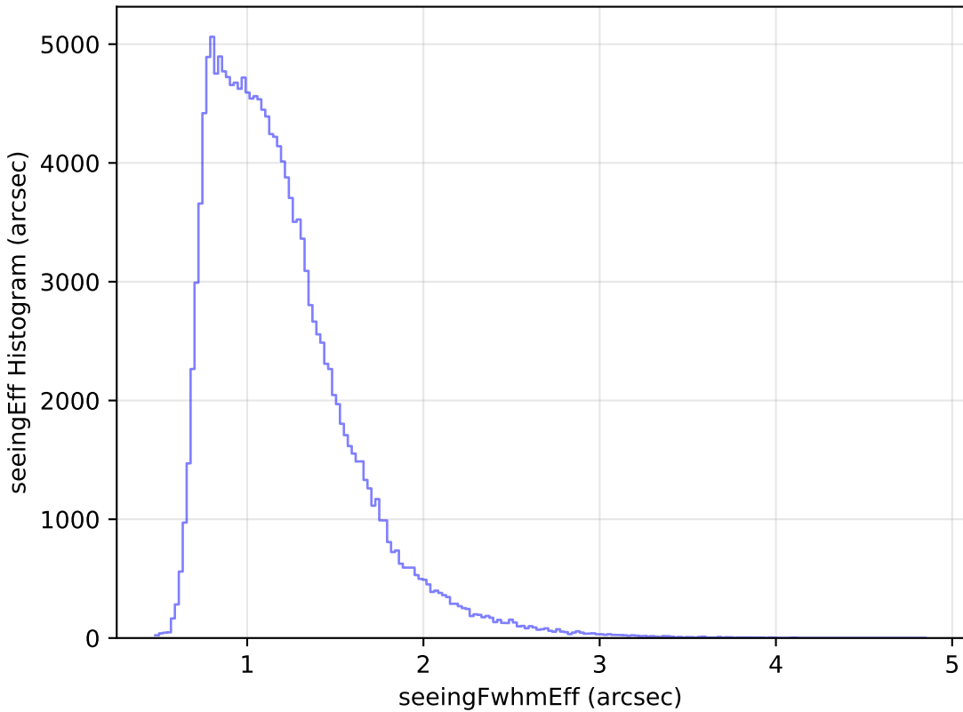
internal_u_expt60_nscale1.5v3.4_10yrs WFD g band: seeingEff Histogram
