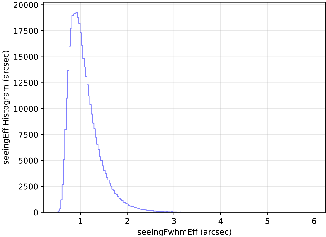
internal_u_expt60_nscale1.5v3.4_10yrs All sky z band: seeingEff Histogram
