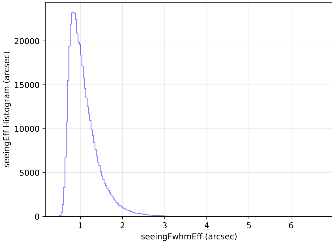
internal_u_expt60_nscale1.5v3.4_10yrs All sky i band: seeingEff Histogram
