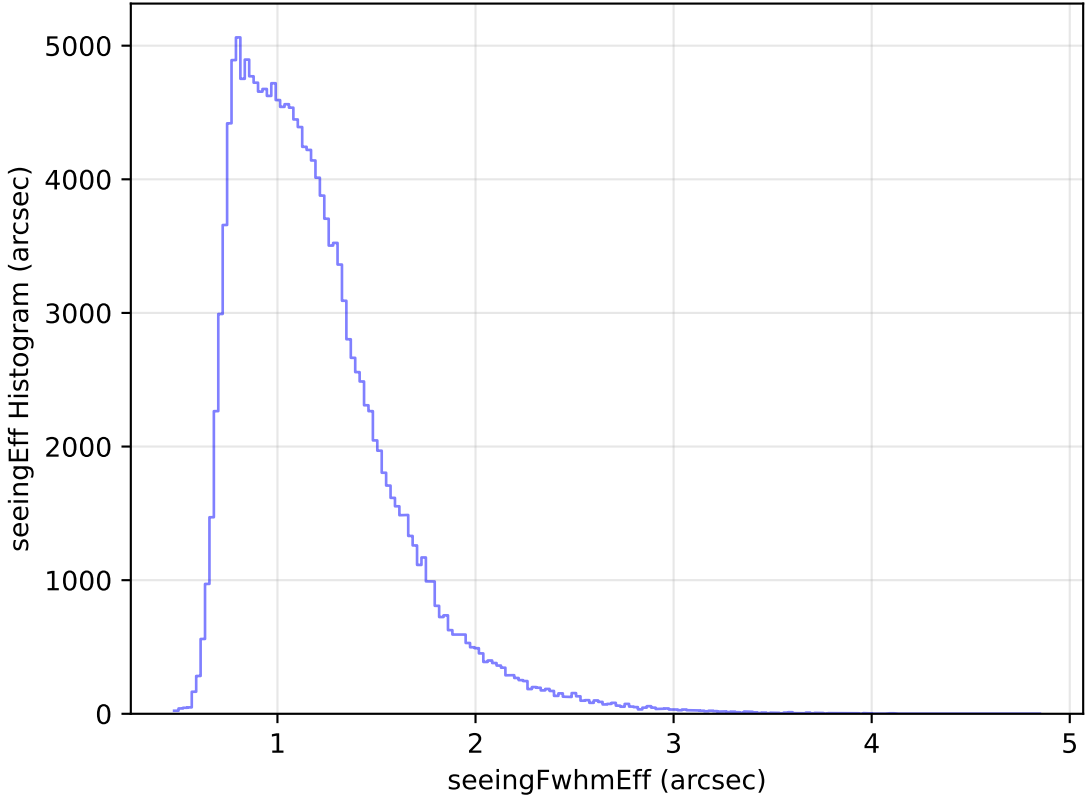
internal_u_expt60_nscale1.5v3.4_10yrs All sky g band: seeingEff Histogram
