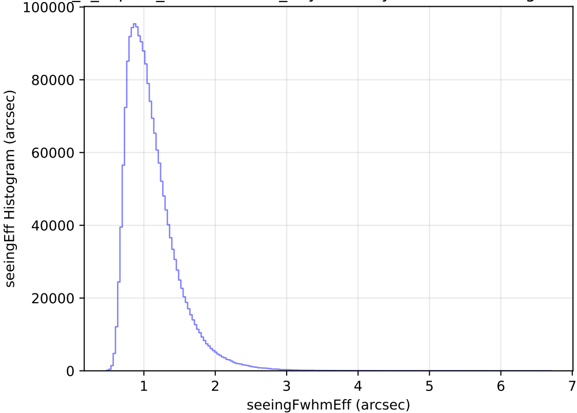
internal_u_expt60_nscale1.5v3.4_10yrs All sky all bands: seeingEff Histogram
