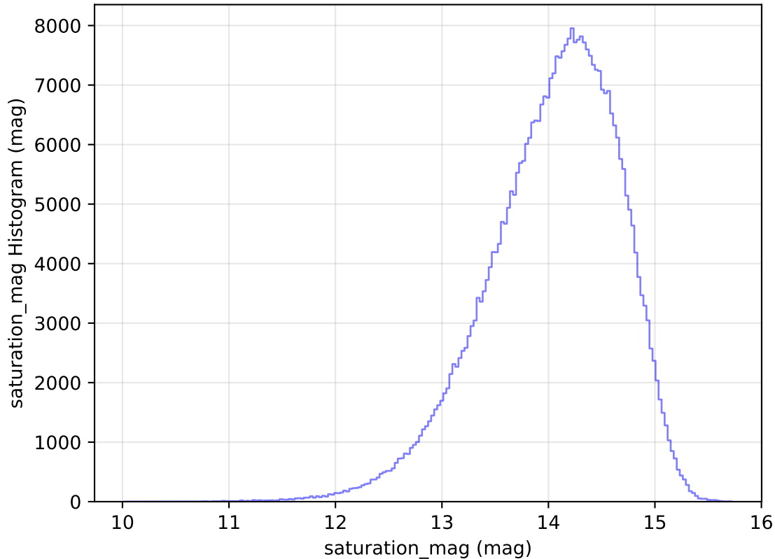
internal_u_expt60_nscale1.5v3.4_10yrs WFD z band: saturation_mag Histogram
