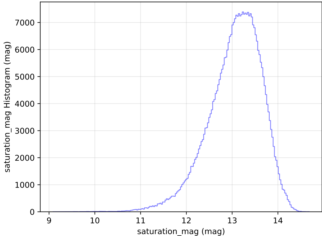
internal_u_expt60_nscale1.5v3.4_10yrs WFD y band: saturation_mag Histogram
