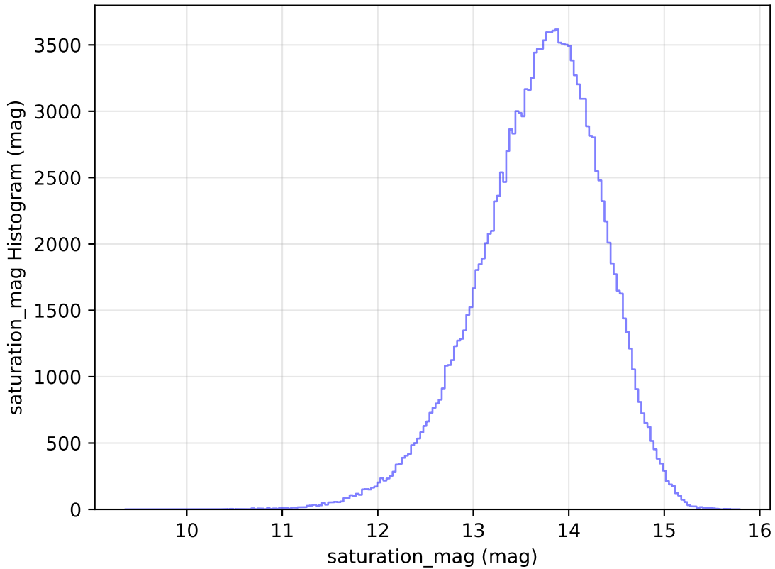
internal_u_expt60_nscale1.5v3.4_10yrs WFD u band: saturation_mag Histogram
