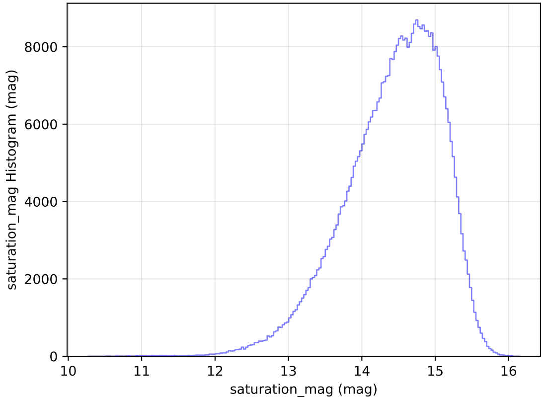
internal_u_expt60_nscale1.5v3.4_10yrs WFD i band: saturation_mag Histogram
