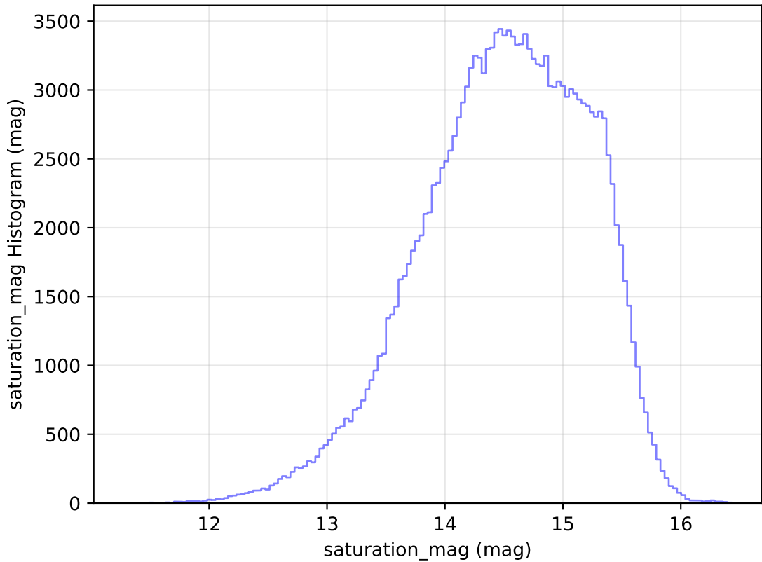
internal_u_expt60_nscale1.5v3.4_10yrs WFD g band: saturation_mag Histogram
