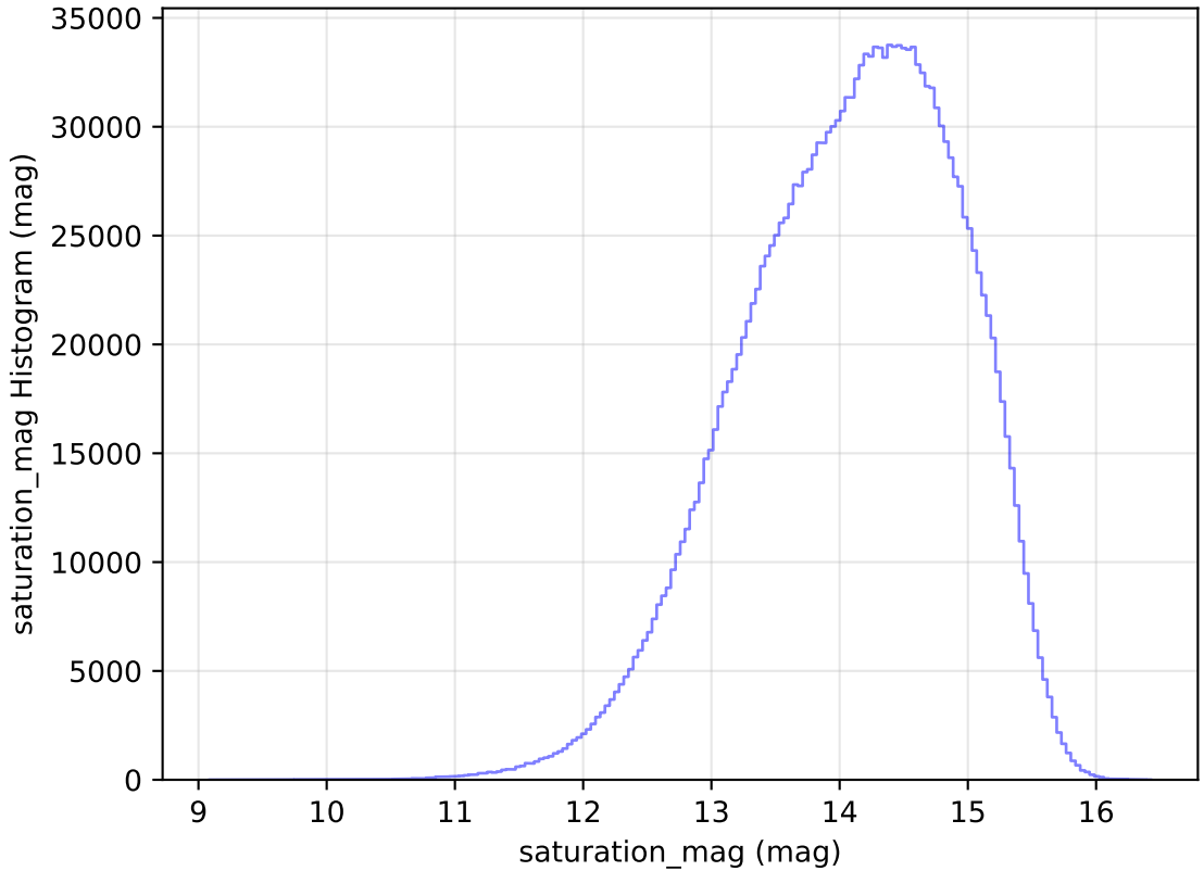
internal_u_expt60_nscale1.5v3.4_10yrs WFD all bands: saturation_mag Histogram
