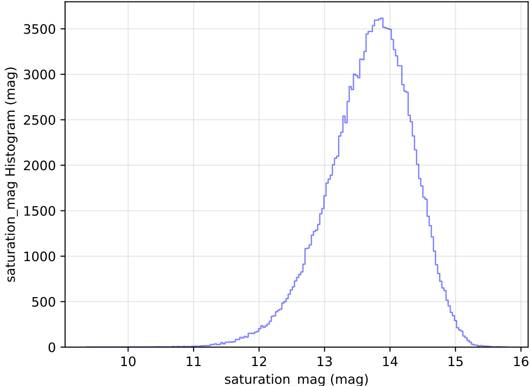
internal_u_expt60_nscale1.5v3.4_10yrs All sky u band: saturation_mag Histogram
