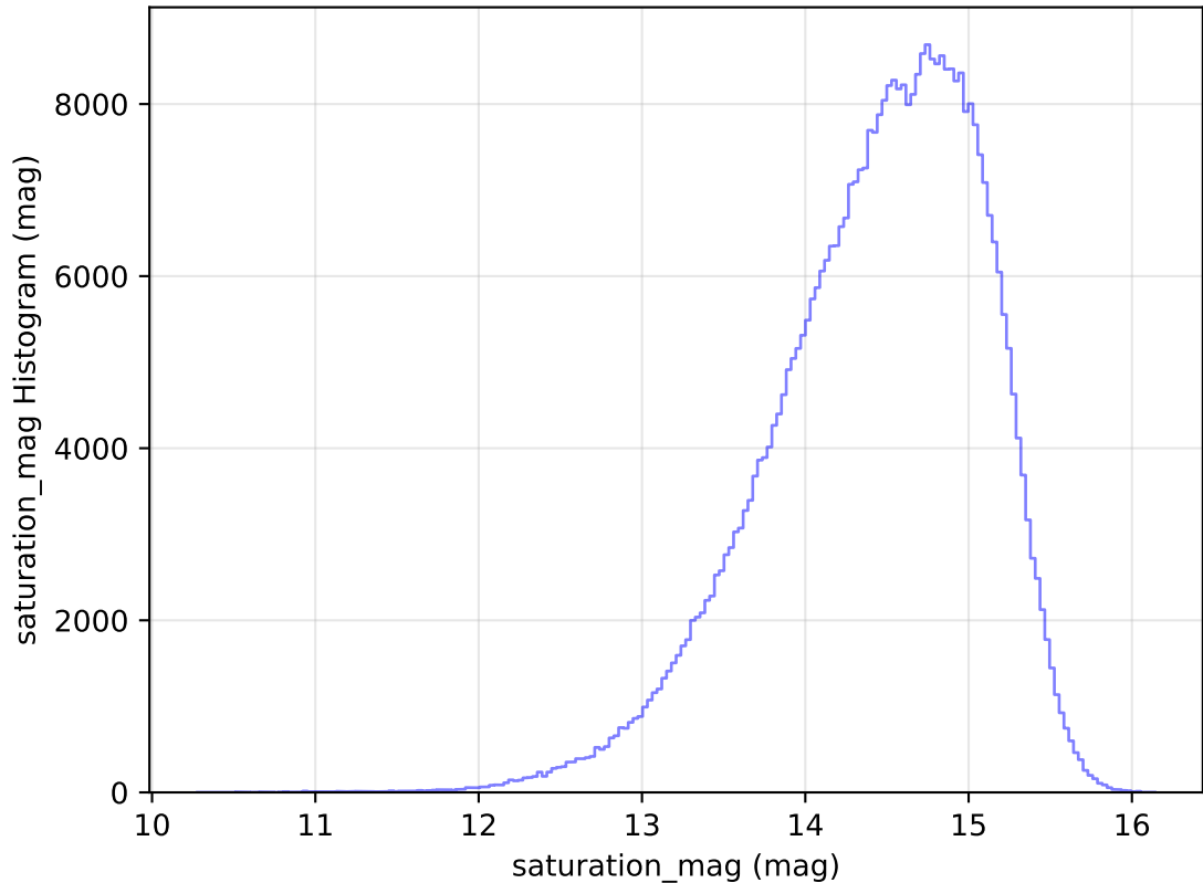
internal_u_expt60_nscale1.5v3.4_10yrs All sky i band: saturation_mag Histogram
