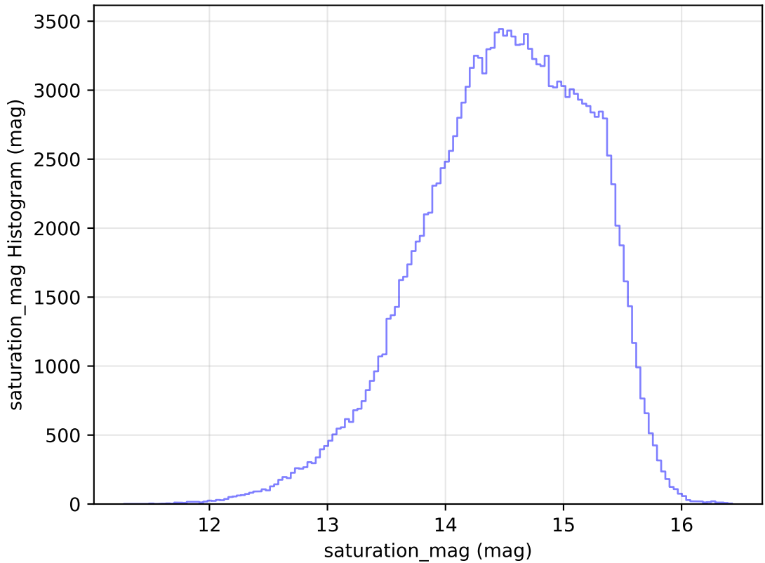
internal_u_expt60_nscale1.5v3.4_10yrs All sky g band: saturation_mag Histogram
