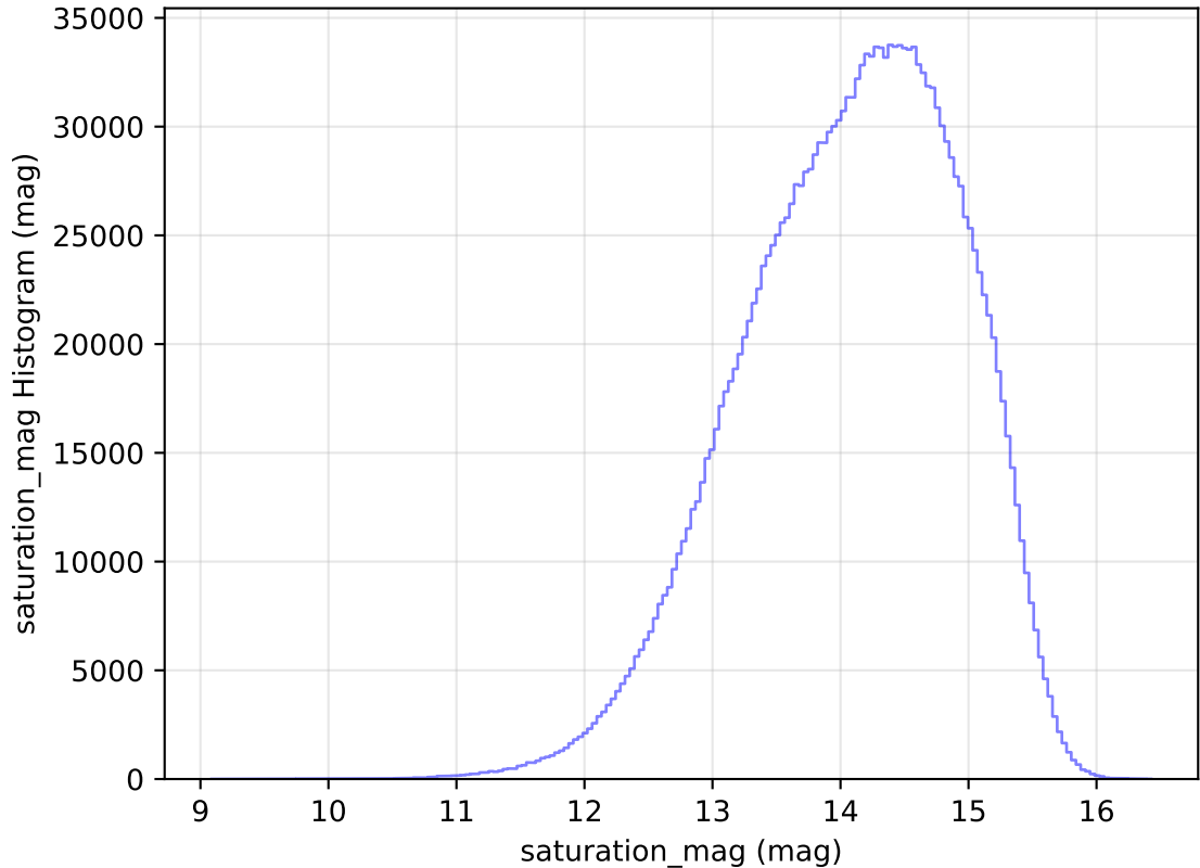
internal_u_expt60_nscale1.5v3.4_10yrs All sky all bands: saturation_mag Histogram
