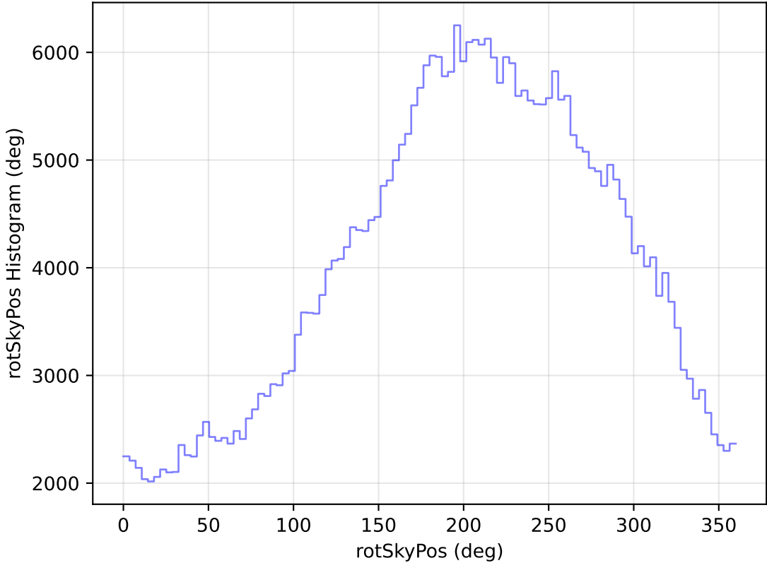
internal_u_expt60_nscale1.5v3.4_10yrs WFD z band: rotSkyPos Histogram
