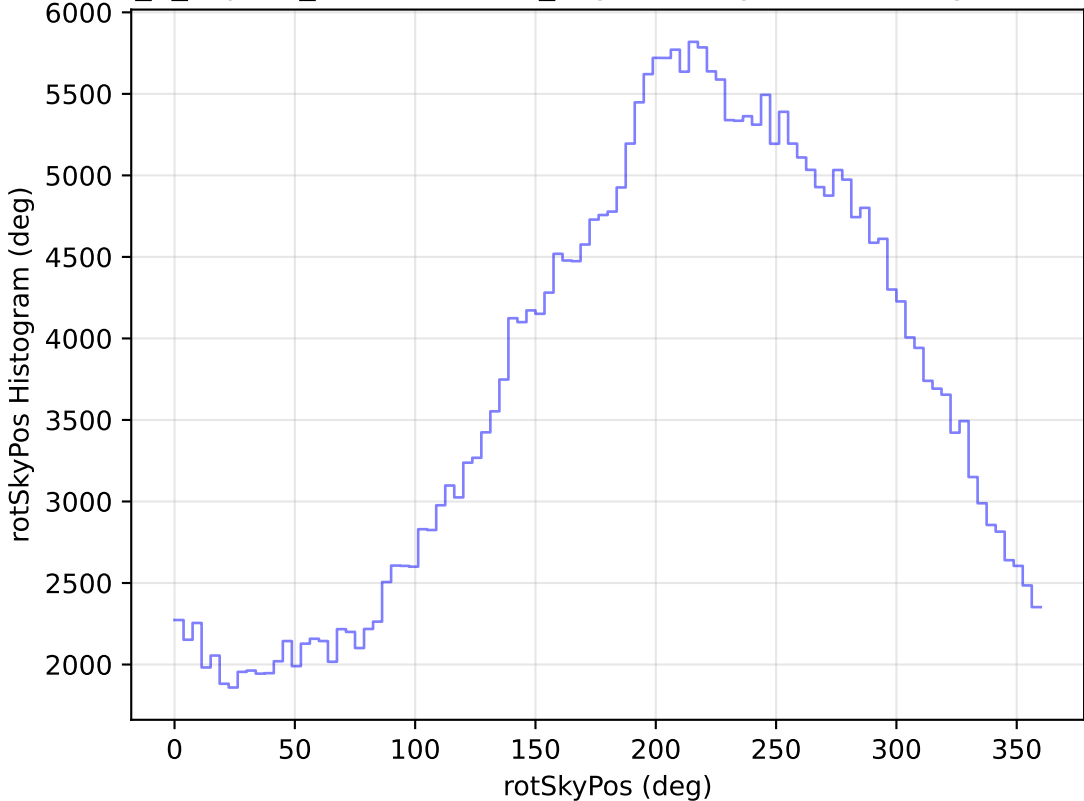
internal_u_expt60_nscale1.5v3.4_10yrs WFD y band: rotSkyPos Histogram
