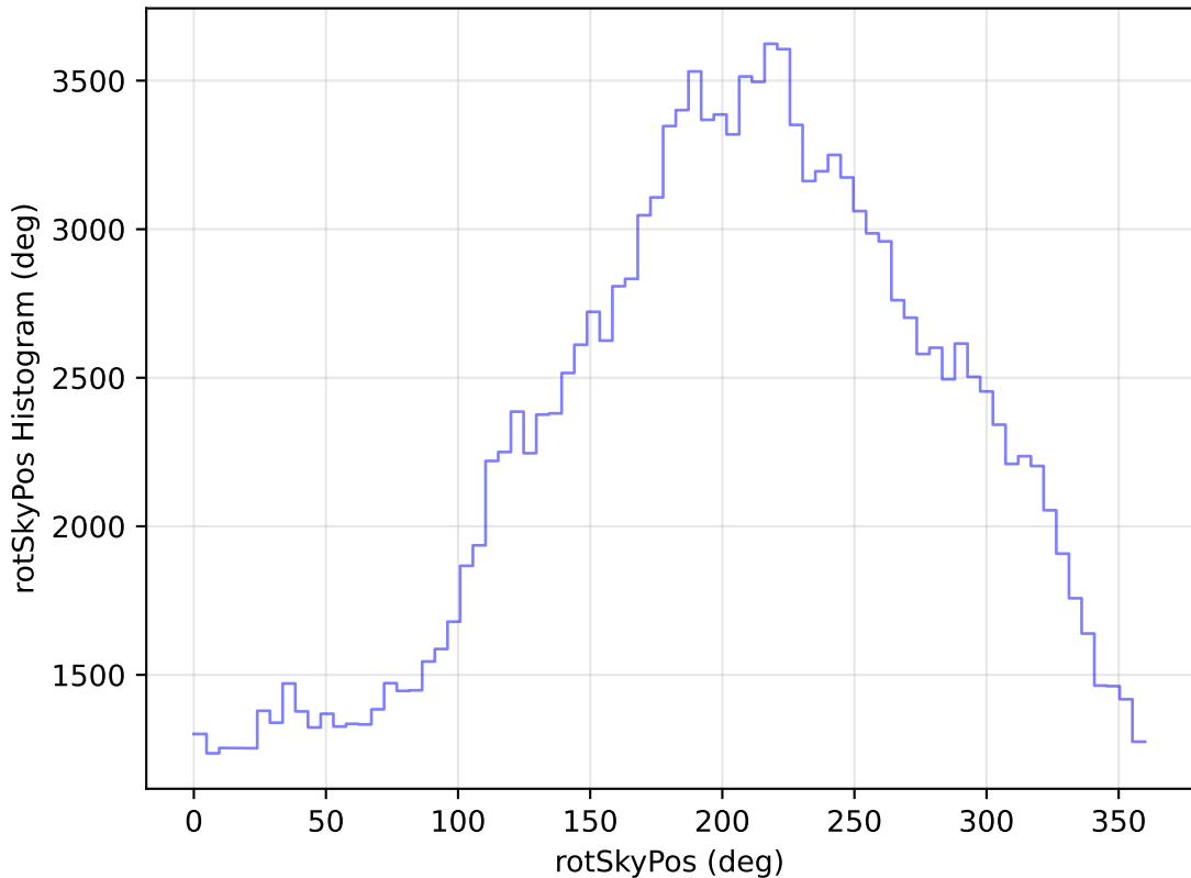
internal_u_expt60_nscale1.5v3.4_10yrs WFD u band: rotSkyPos Histogram
