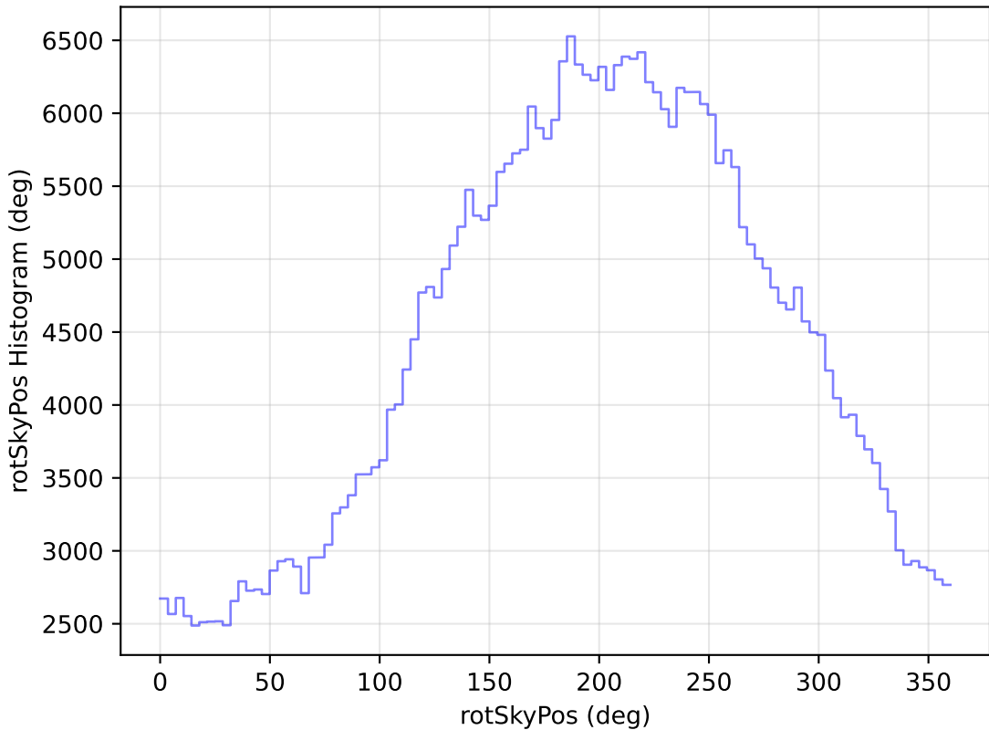
internal_u_expt60_nscale1.5v3.4_10yrs WFD r band: rotSkyPos Histogram
