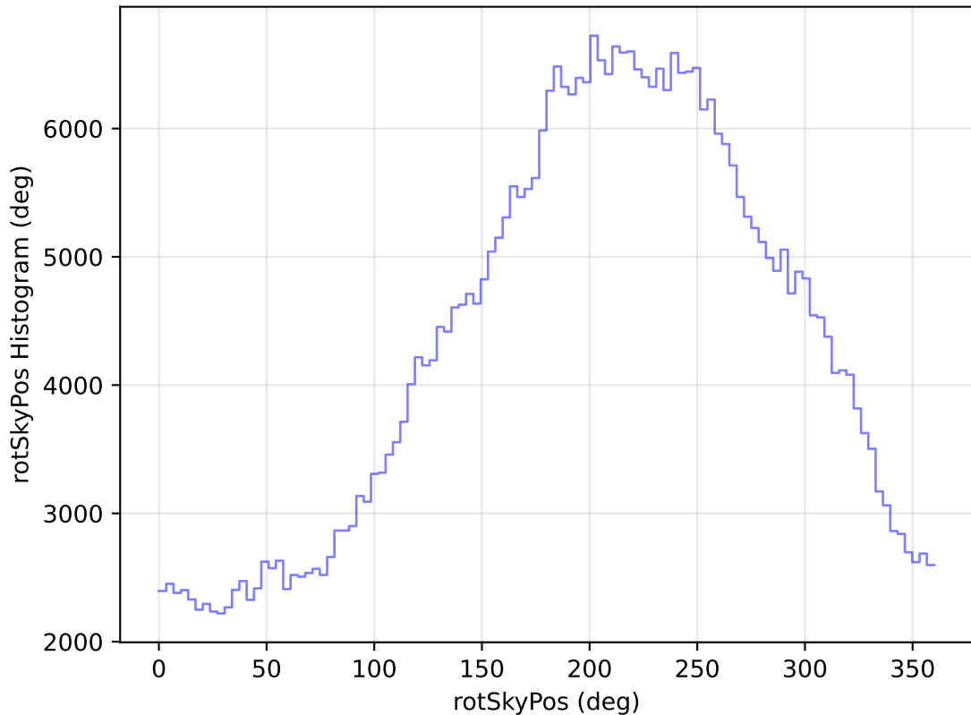
internal_u_expt60_nscale1.5v3.4_10yrs WFD i band: rotSkyPos Histogram
