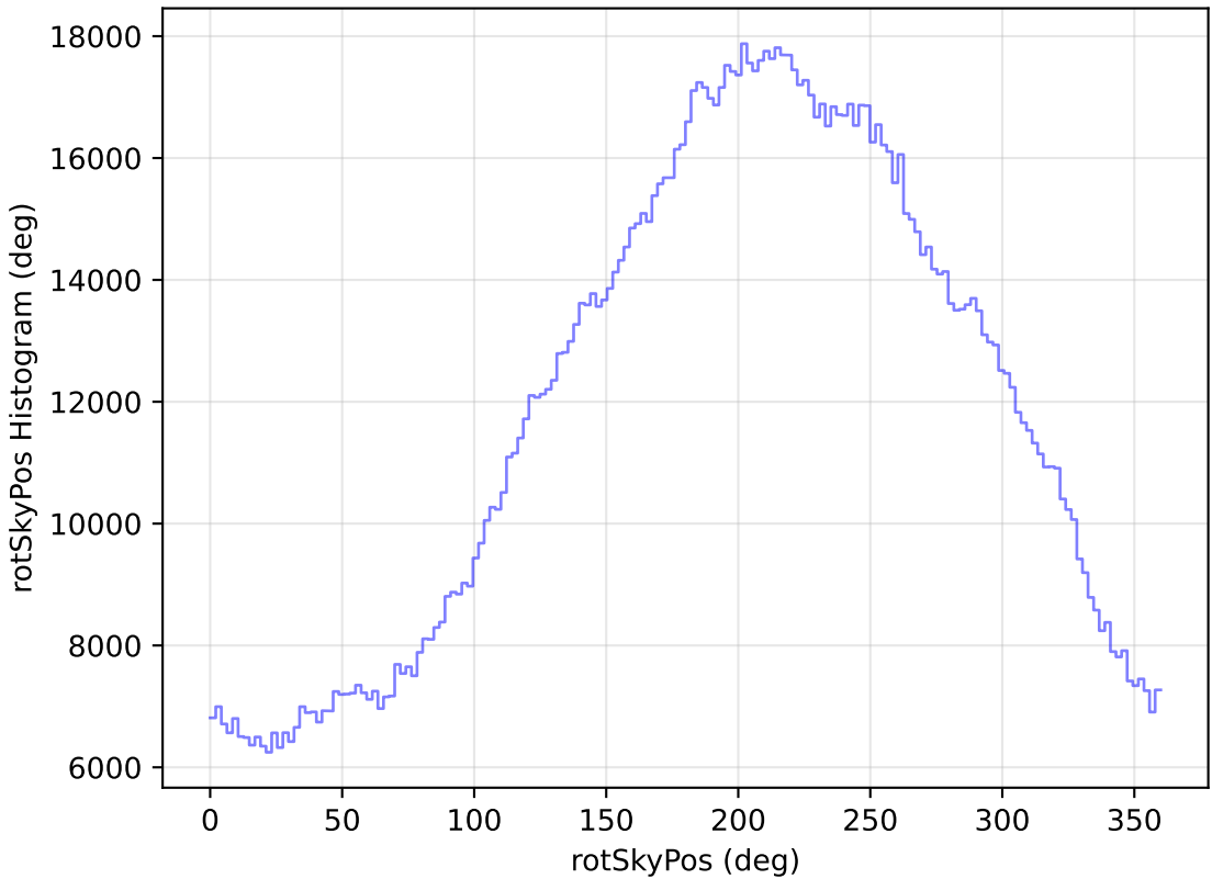
internal_u_expt60_nscale1.5v3.4_10yrs WFD all bands: rotSkyPos Histogram
