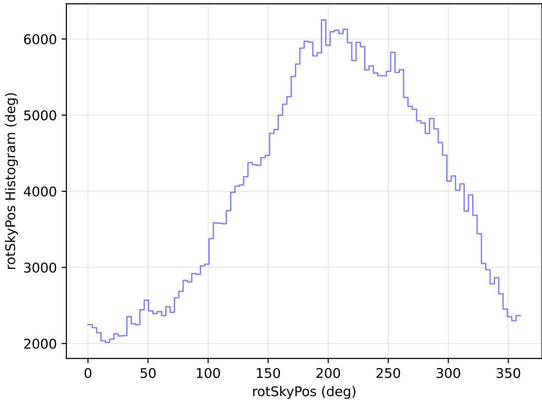
internal_u_expt60_nscale1.5v3.4_10yrs All sky z band: rotSkyPos Histogram
