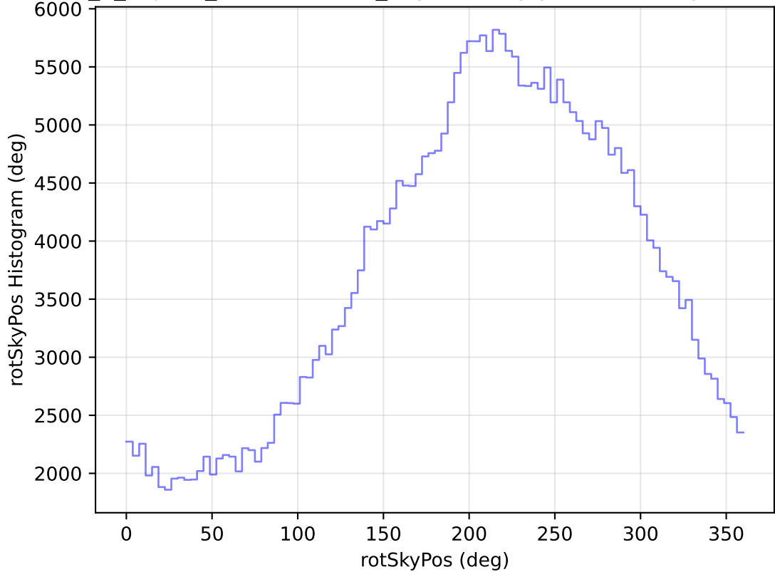
internal_u_expt60_nscale1.5v3.4_10yrs All sky y band: rotSkyPos Histogram
