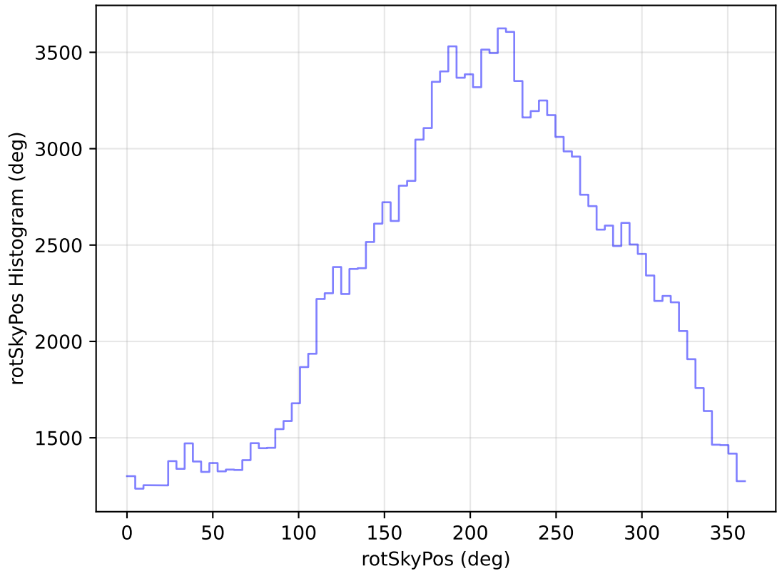
internal_u_expt60_nscale1.5v3.4_10yrs All sky u band: rotSkyPos Histogram
