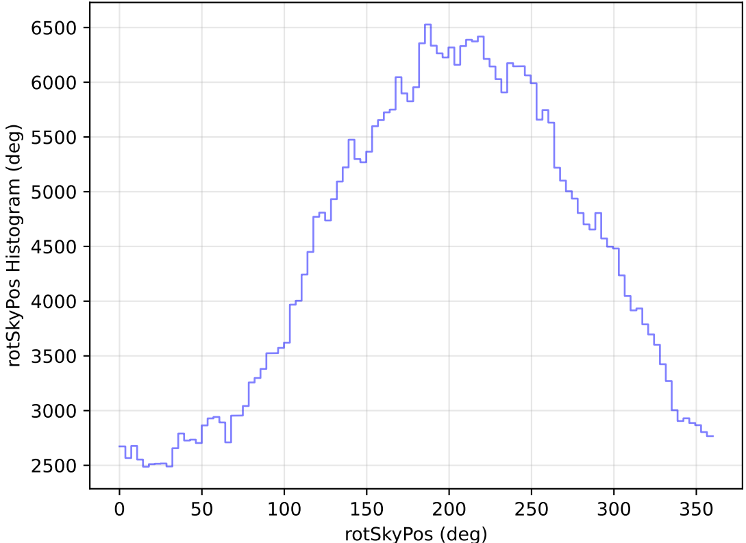
internal_u_expt60_nscale1.5v3.4_10yrs All sky r band: rotSkyPos Histogram
