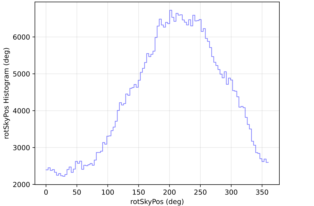
internal_u_expt60_nscale1.5v3.4_10yrs All sky i band: rotSkyPos Histogram
