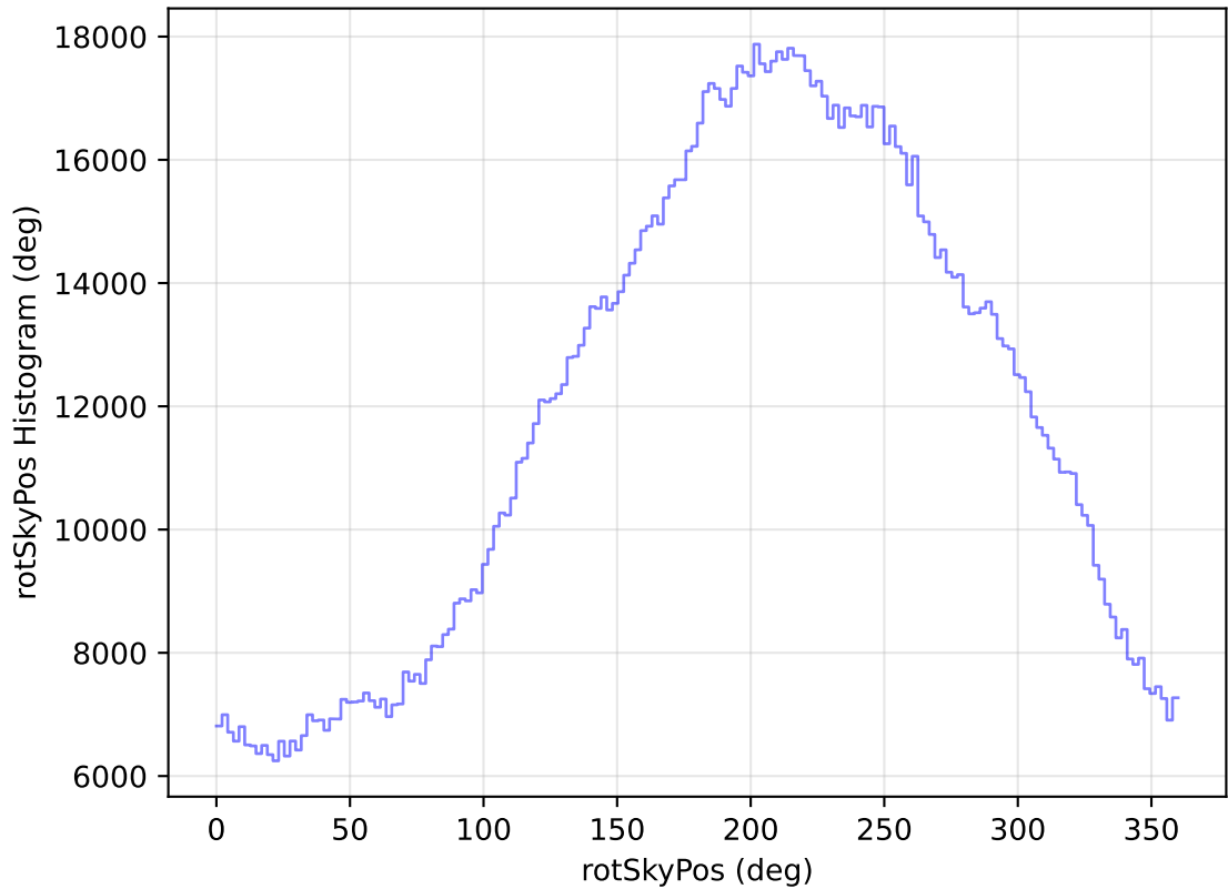
internal_u_expt60_nscale1.5v3.4_10yrs All sky all bands: rotSkyPos Histogram
