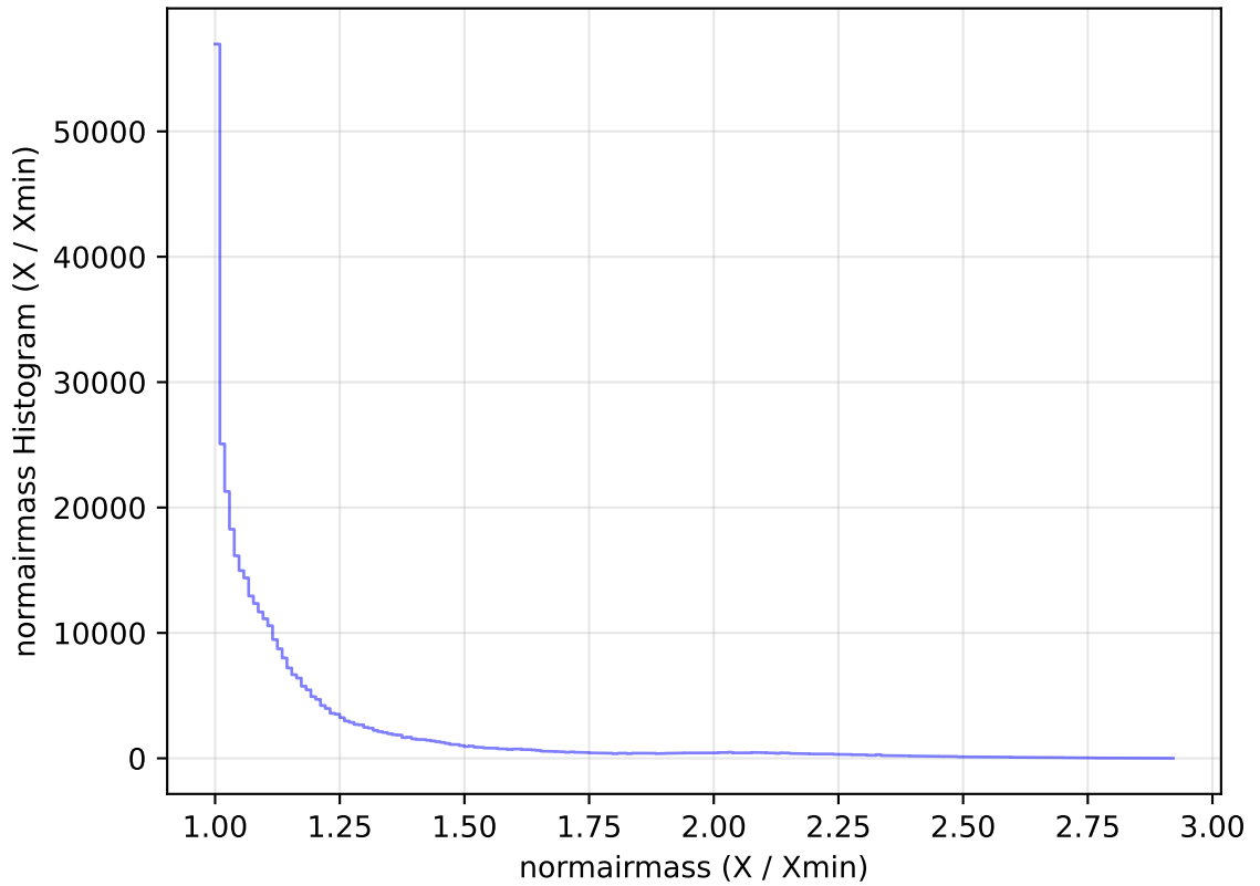
internal_u_expt60_nscale1.5v3.4_10yrs WFD z band: normairmass Histogram
