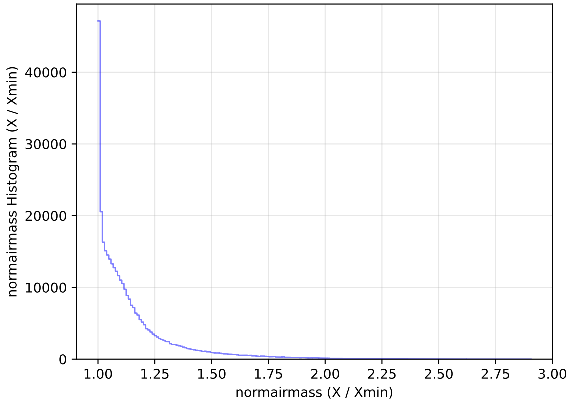
internal_u_expt60_nscale1.5v3.4_10yrs WFD y band: normairmass Histogram
