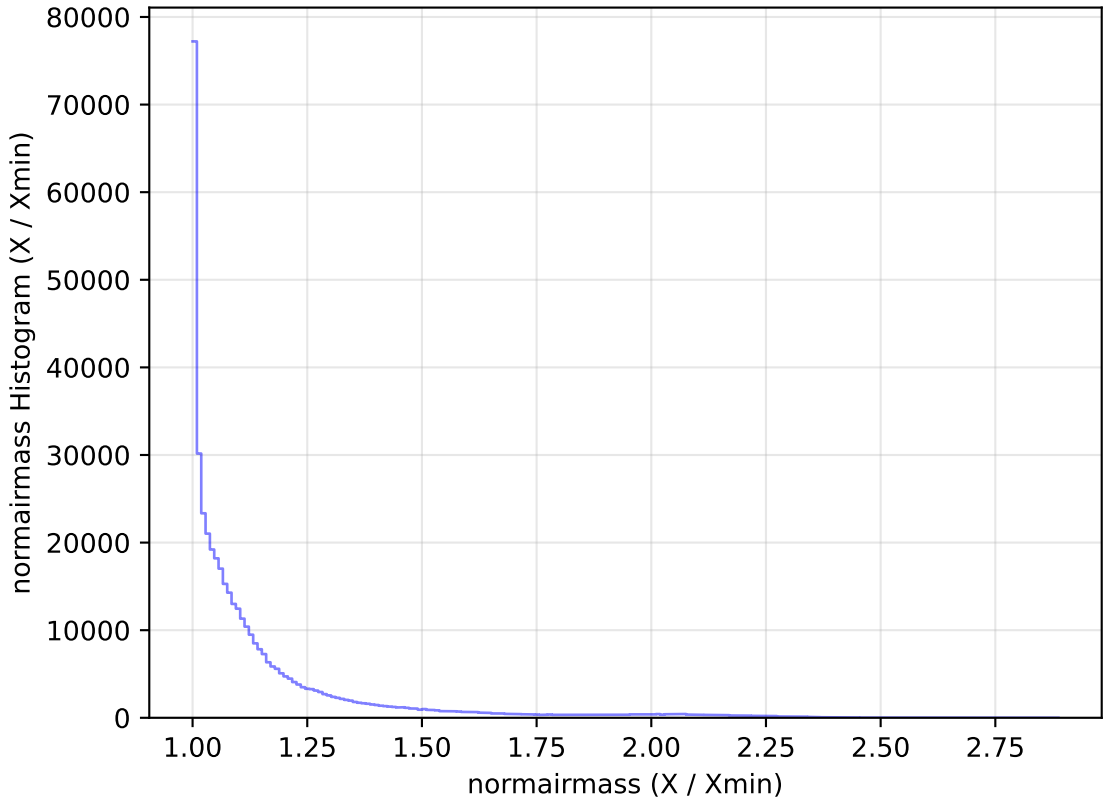
internal_u_expt60_nscale1.5v3.4_10yrs WFD r band: normairmass Histogram
