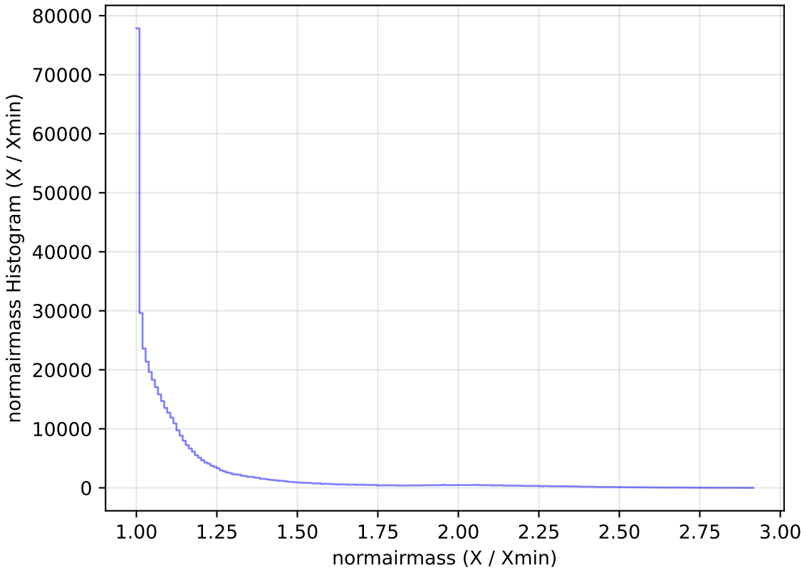
internal_u_expt60_nscale1.5v3.4_10yrs WFD i band: normairmass Histogram
