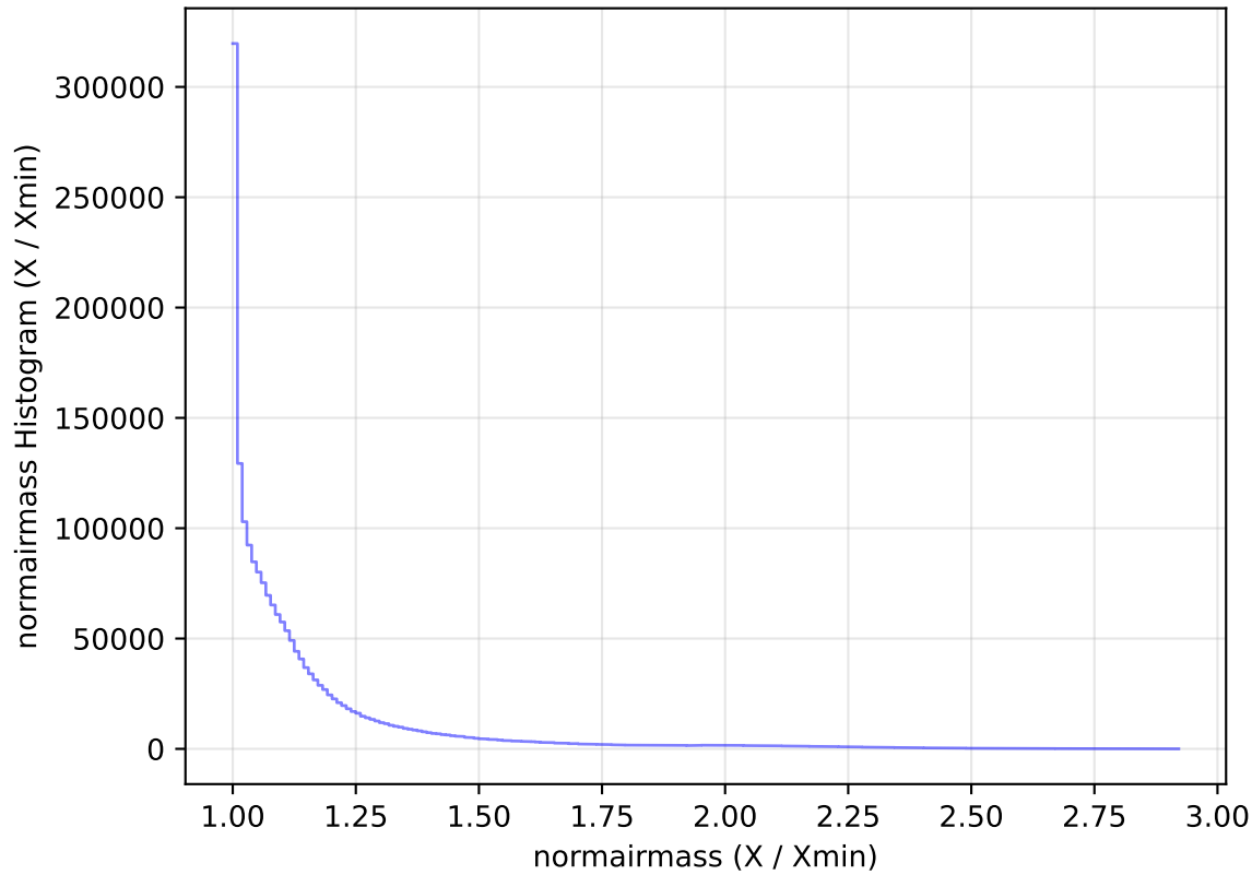
internal_u_expt60_nscale1.5v3.4_10yrs WFD all bands: normairmass Histogram
