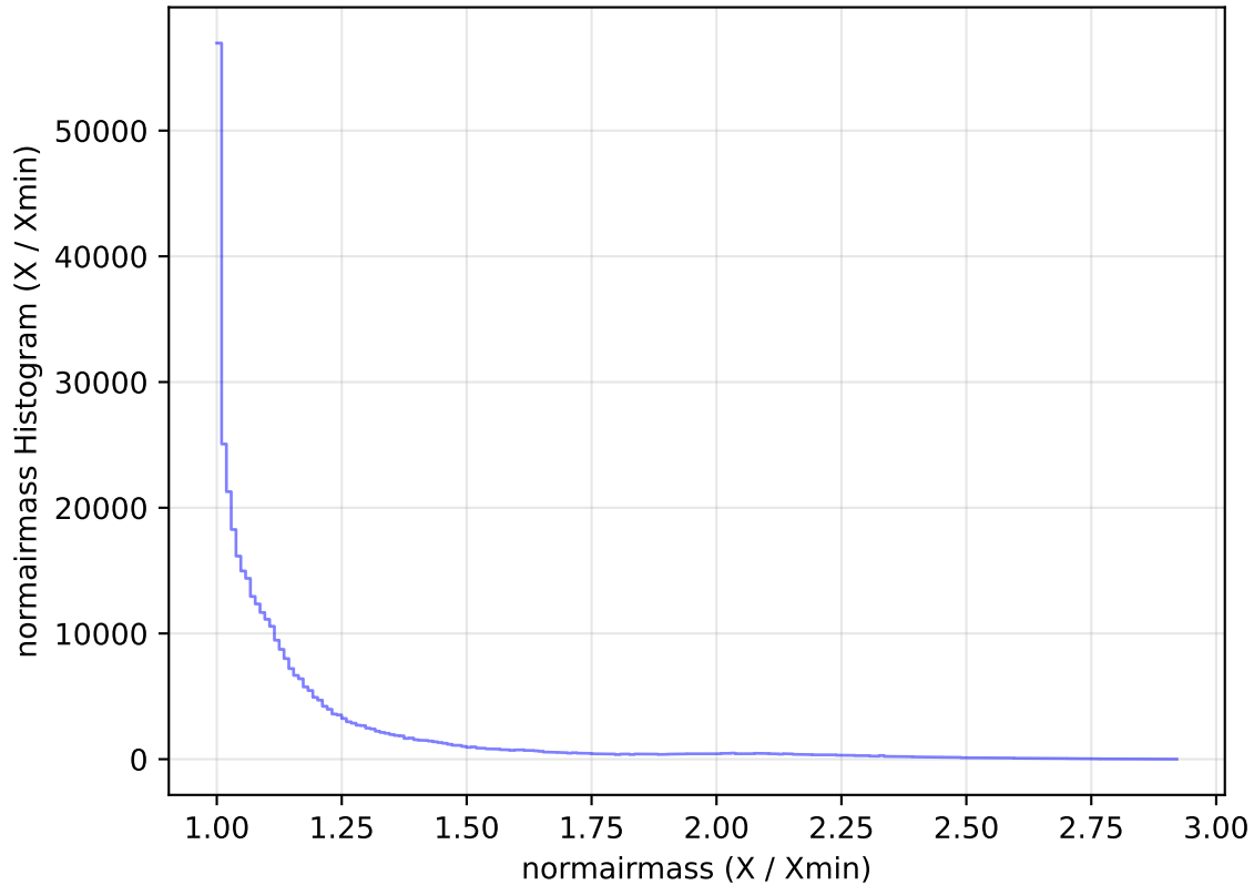
internal_u_expt60_nscale1.5v3.4_10yrs All sky z band: normairmass Histogram
