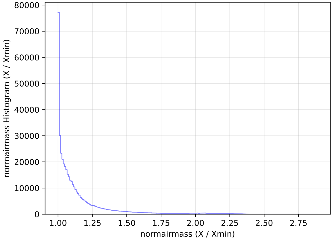
internal_u_expt60_nscale1.5v3.4_10yrs All sky r band: normairmass Histogram
