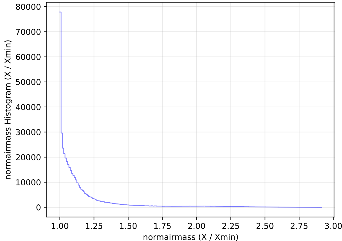
internal_u_expt60_nscale1.5v3.4_10yrs All sky i band: normairmass Histogram
