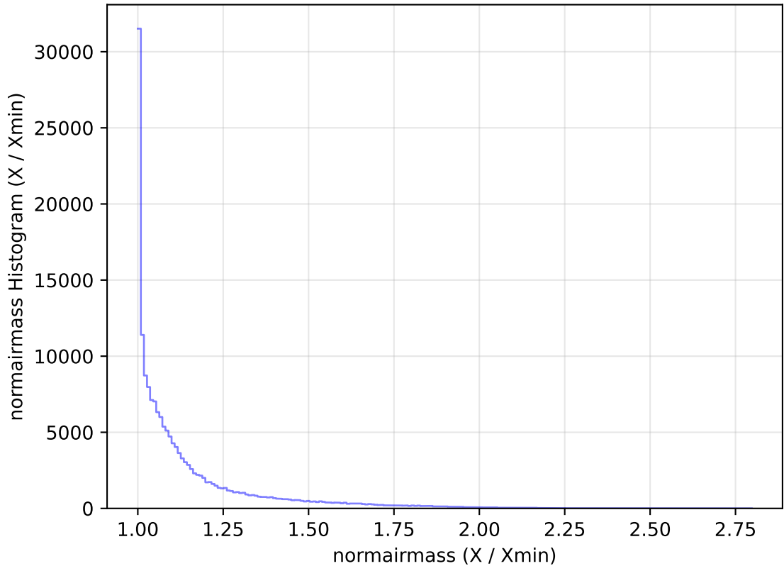
internal_u_expt60_nscale1.5v3.4_10yrs All sky g band: normairmass Histogram
