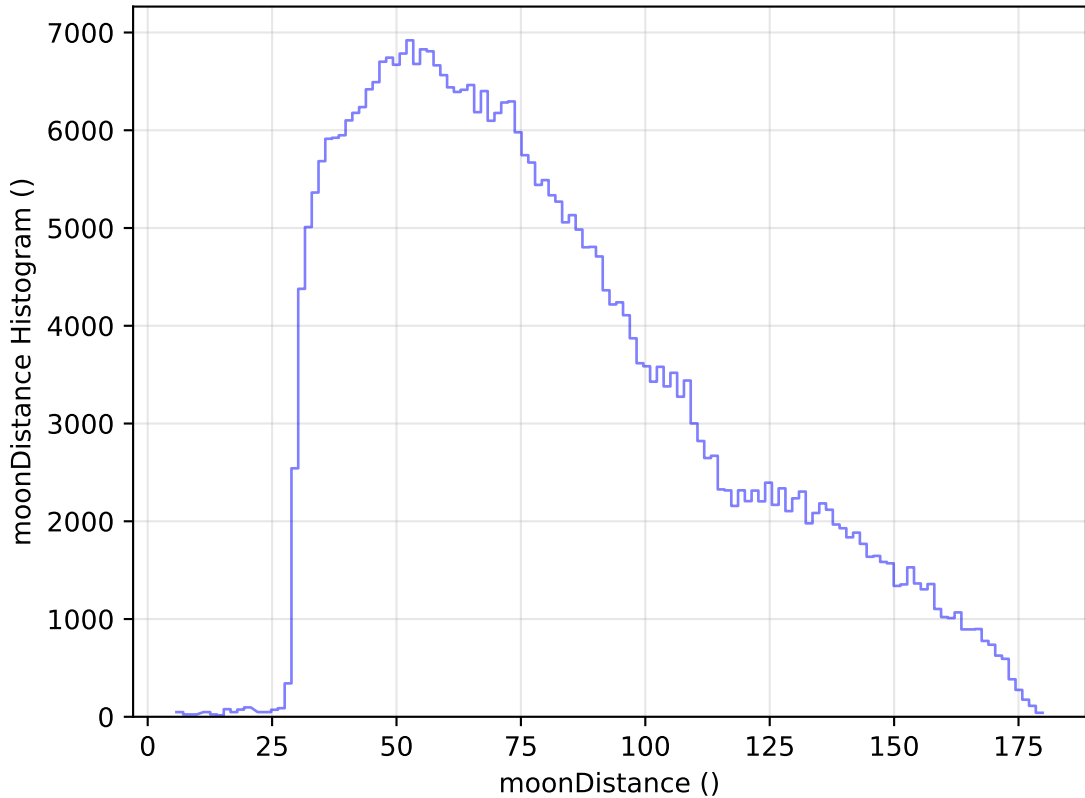
internal_u_expt60_nscale1.5v3.4_10yrs WFD z band: moonDistance Histogram
