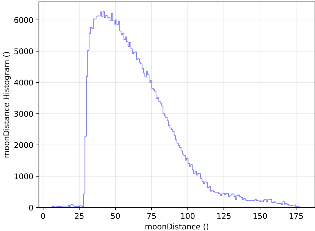
internal_u_expt60_nscale1.5v3.4_10yrs WFD y band: moonDistance Histogram
