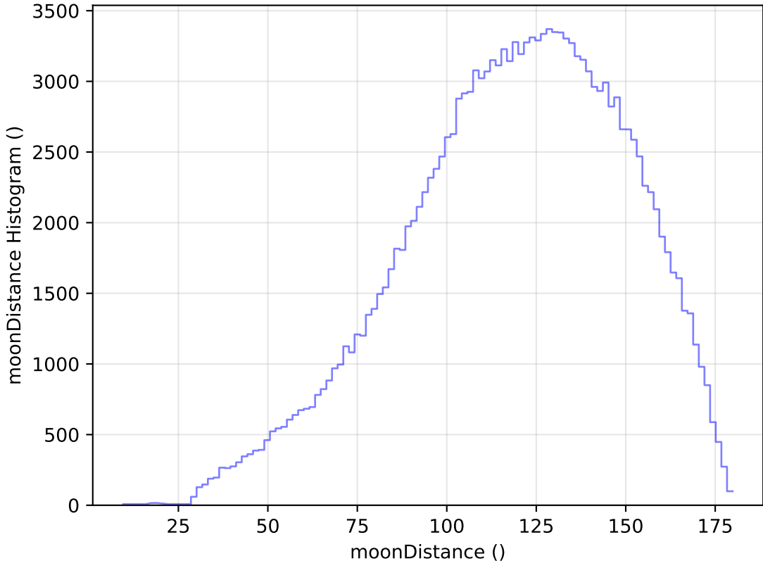
internal_u_expt60_nscale1.5v3.4_10yrs WFD u band: moonDistance Histogram
